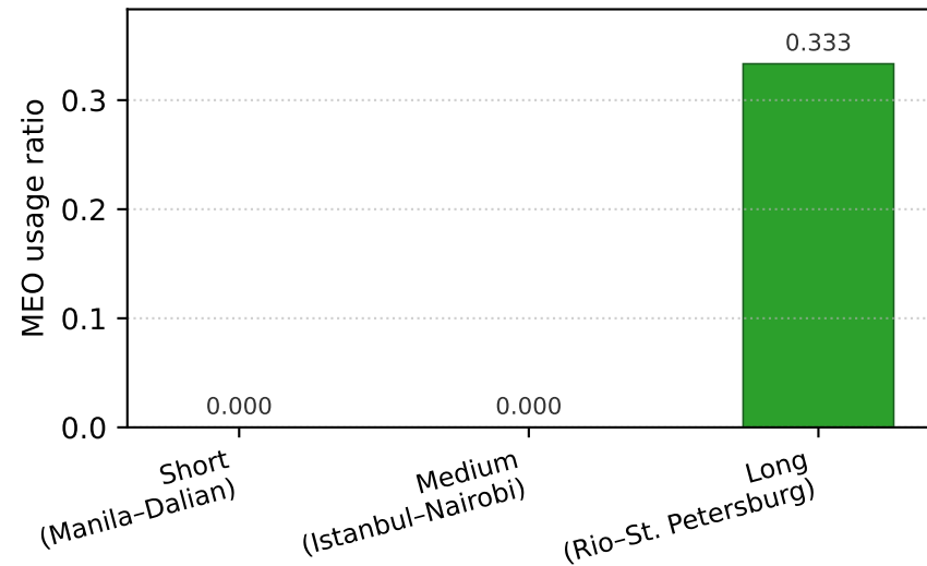
(a) MEO usage ratio
